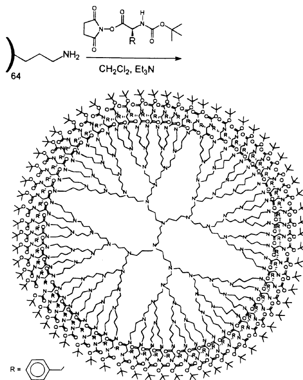
Fig. 9 A dendritic box capable of encapsulating small guest molecules during construction. (Reproduced with permission from J. Am. Chem. Soc. , 1995, 117 , 4417.)
